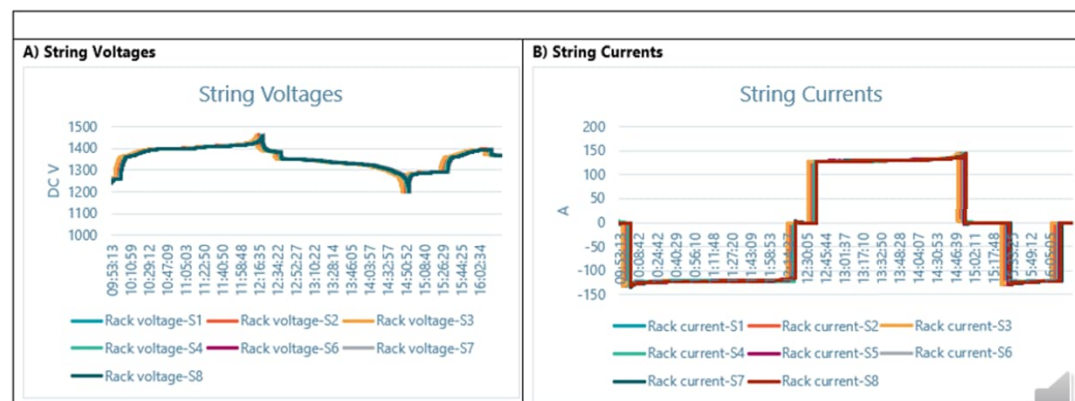
Figure 2-3: String Voltages and Currents
